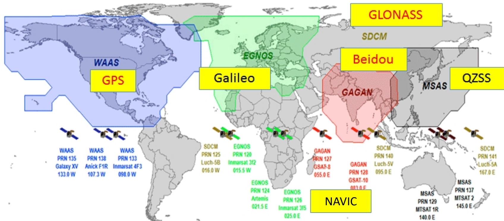
GNSS constellations, augmentations, and regional constellations [7]
