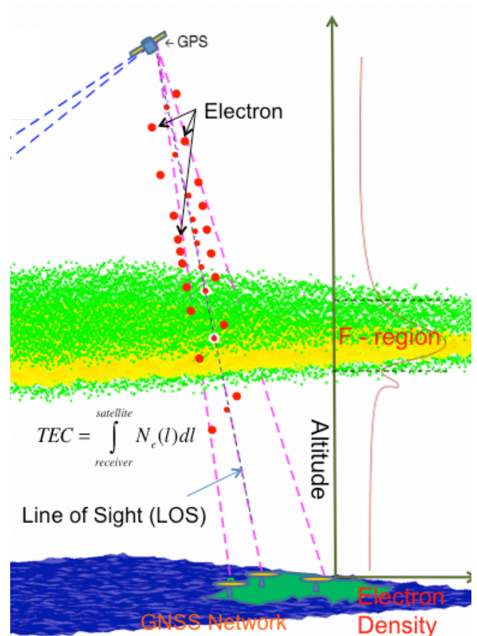
Ground-based measurement of ionospheric disturbance [28]
