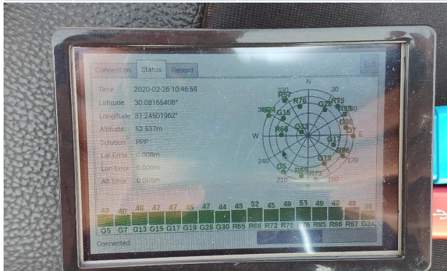
MADOCA PPP measurement display on RaspberryPi device.
