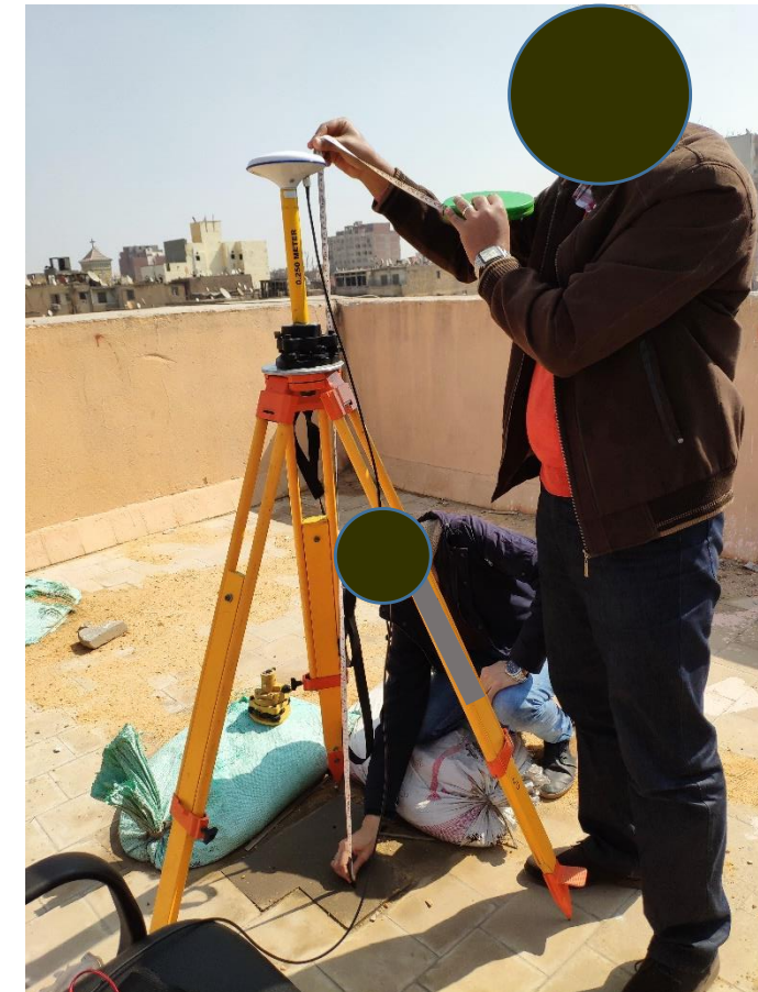
Measuring antenna height from the ground control point for precise measurement.
